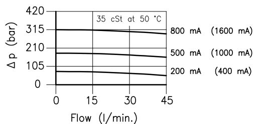
Type T (14–315 bar)
