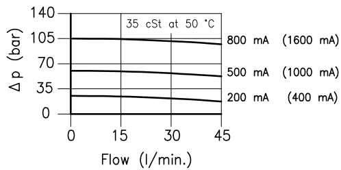
Type U (7–105 bar)
