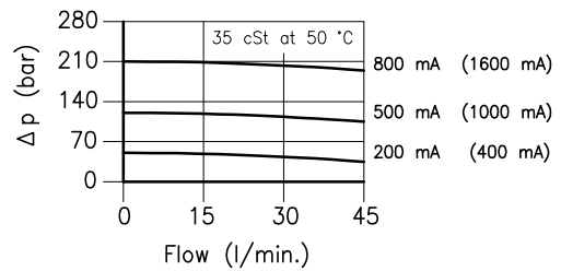
Type D (10–210 bar)
